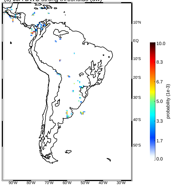
(c) JJA DWC strong thresholds (uw)
