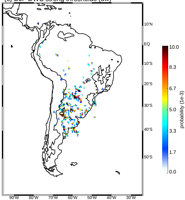
(c) DJF DWC strong thresholds (uw)
