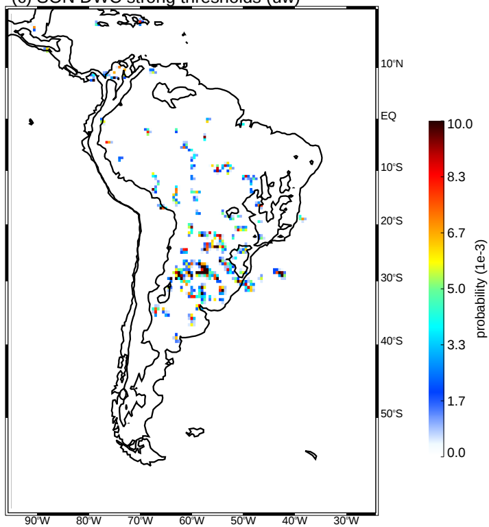
(c) SON DWC strong thresholds (uw)
