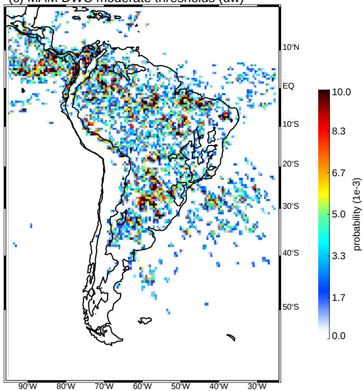
(c) MAM DWC moderate thresholds (uw)
