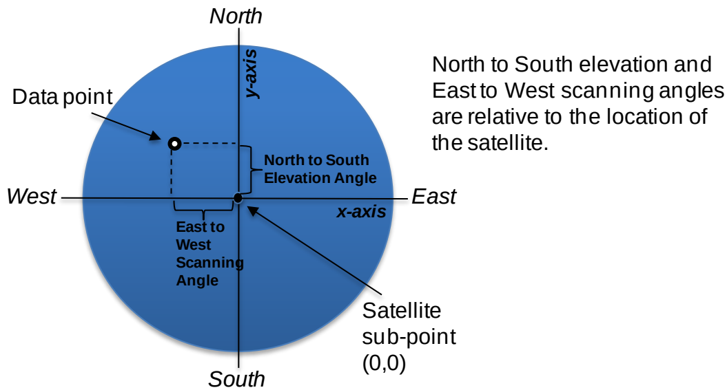
Figure 7.1.2.2-1 ABI Fixed Grid Coordinate System
