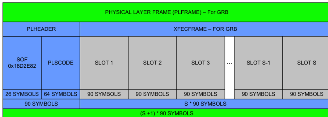
Figure 4.3.1 GRB DVB-S2 Physical Layer Framing
