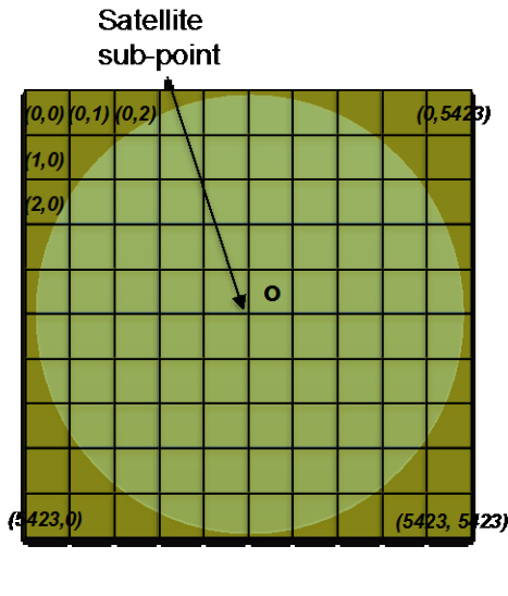
Figure 7.1.2.6-2 Relating a Data Point to Its ABI Fixed Grid Coordinates
