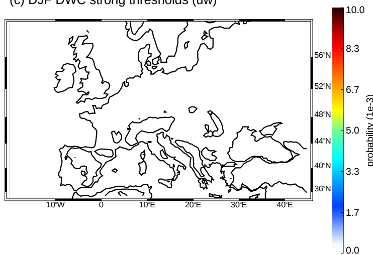
(c) DJF DWC strong thresholds (uw)
