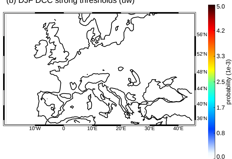
(b) DJF DCC strong thresholds (uw)
