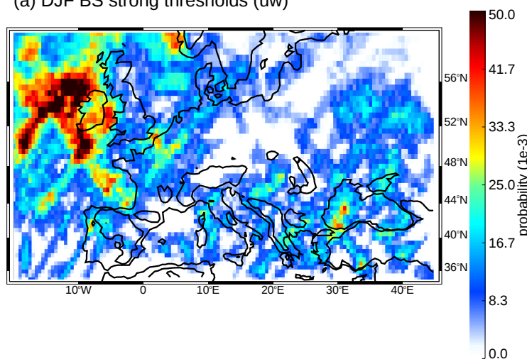
(a) DJF BS strong thresholds (uw)
