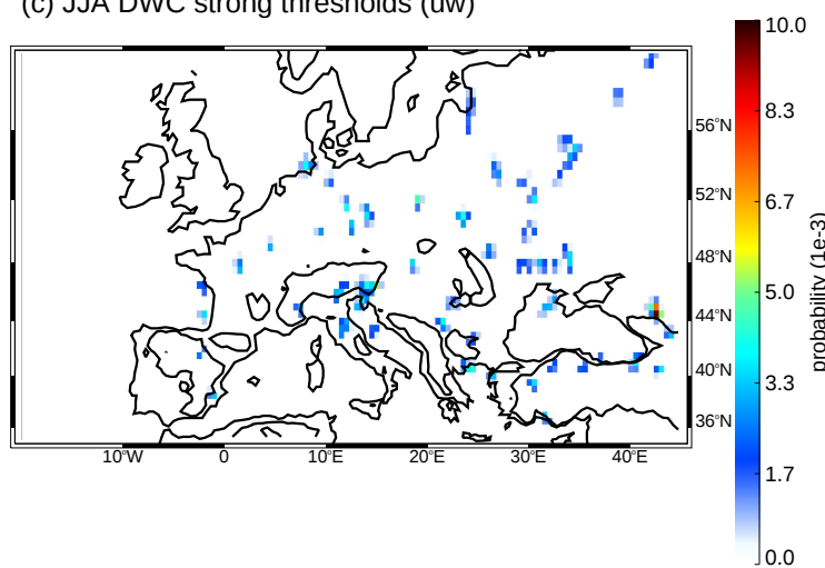
(c) JJA DWC strong thresholds (uw)
