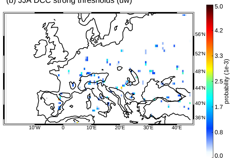
(b) JJA DCC strong thresholds (uw)
