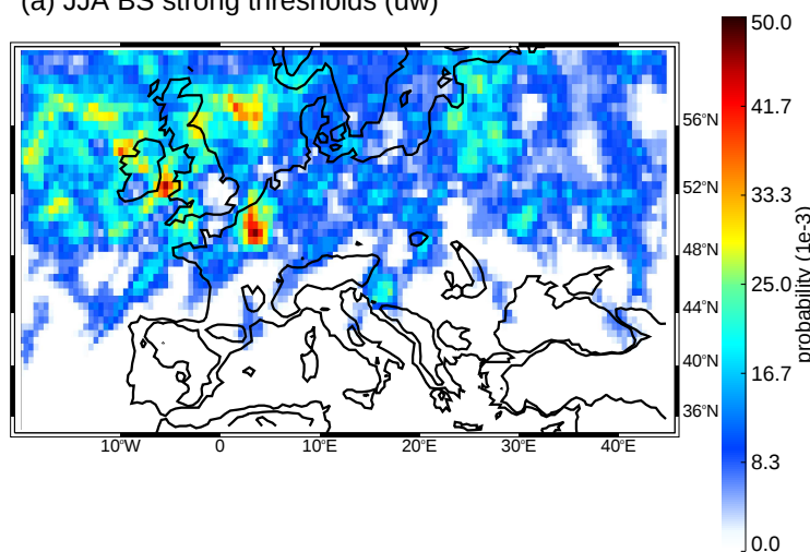
(a) JJA BS strong thresholds (uw)
