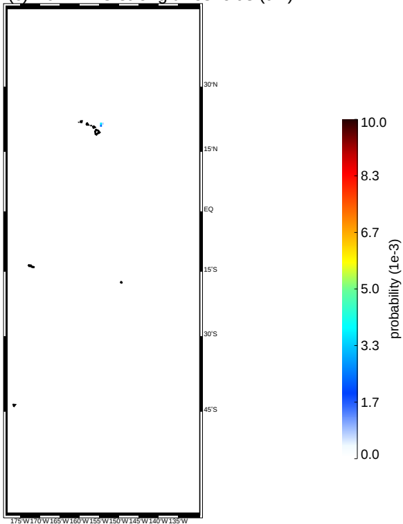
(c) DJF DWC strong thresholds (uw)
