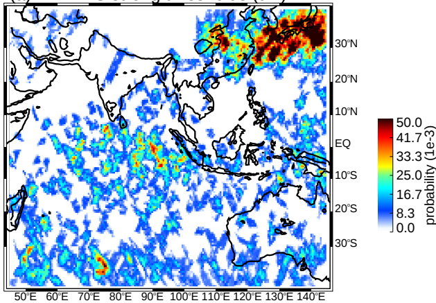
(a) MAM BS strong thresholds (uw)
