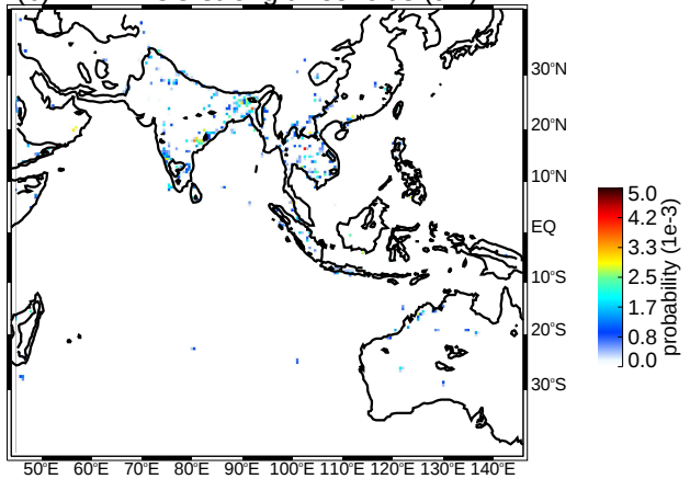
(b) MAM DCC strong thresholds (uw)
