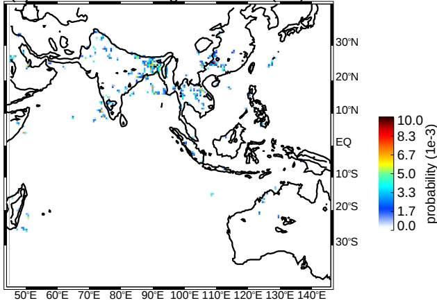
(c) MAM DWC strong thresholds (uw)
