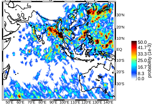
(c) JJA DWC strong thresholds (uw)
