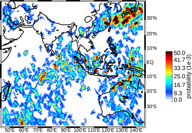
(a) DJF BS strong thresholds (uw)
