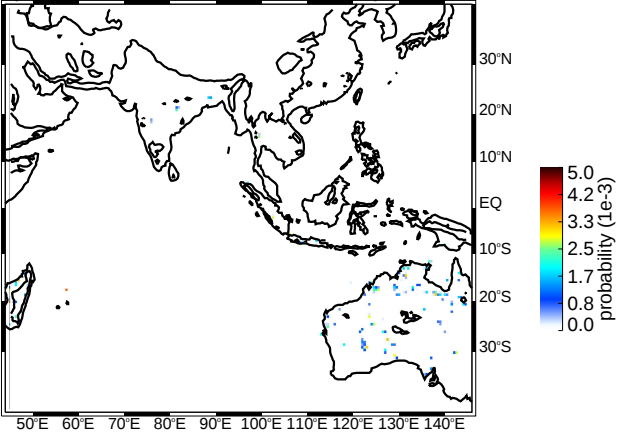
(b) DJF DCC strong thresholds (uw)
