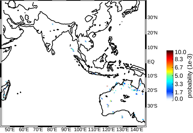
(c) DJF DWC strong thresholds (uw)
