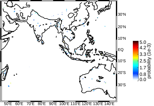
(b) SON DCC strong thresholds (uw)
