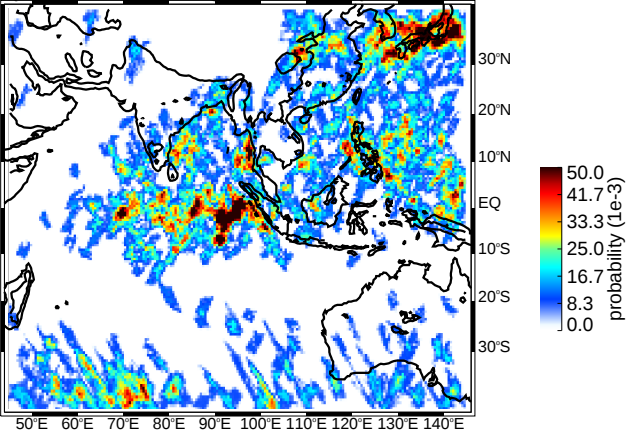
(a) SON BS strong thresholds (uw)
