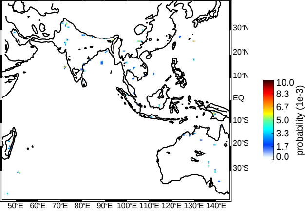
(c) SON DWC strong thresholds (uw)
