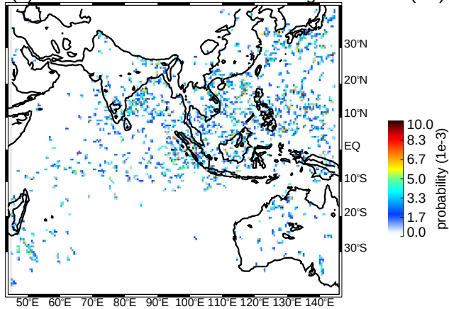
(e) SON wide convective cores strong thresholds (uw)
