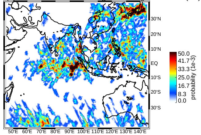
(f) SON broad strat regions between mod & str thresholds (uw)
