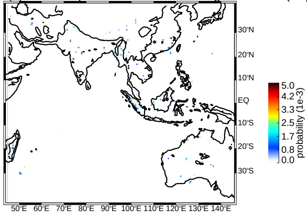
(c) SON deep/wide convective cores strong thresholds (uw)
