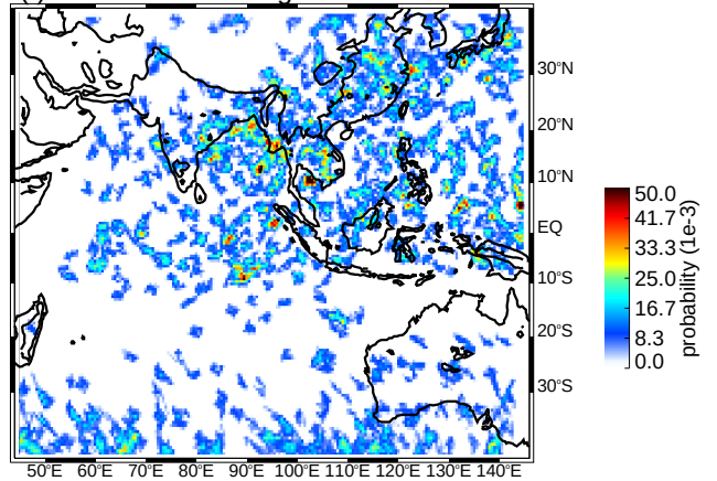
(f) JJA broad strat regions between mod & str thresholds (uw)
