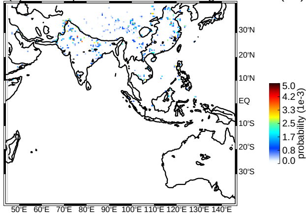
(c) JJA deep/wide convective cores strong thresholds (uw)
