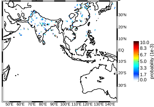
(e) JJA wide convective cores strong thresholds (uw)
