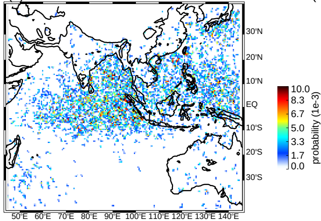
(e) SON wide convective cores moderate thresholds (uw)
