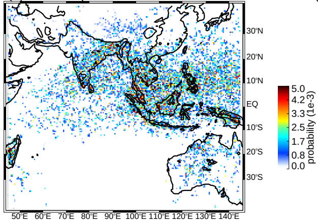
(c) SON deep/wide convective cores moderate thresholds (uw)
