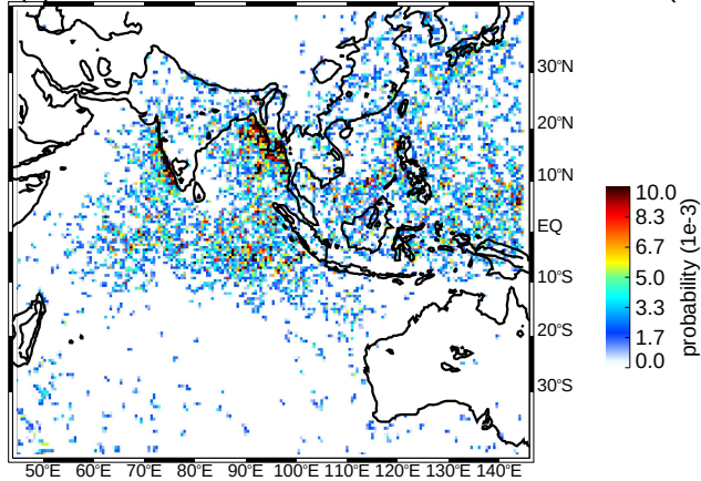
(e) JJA wide convective cores moderate thresholds (uw)
