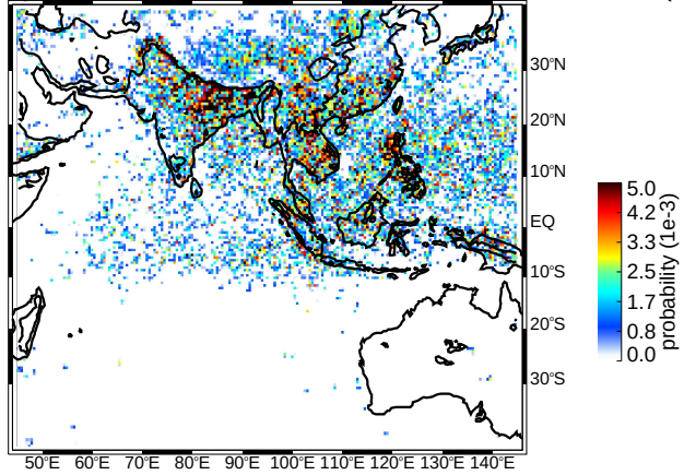
(c) JJA deep/wide convective cores moderate thresholds (uw)
