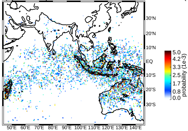
(c) DJF deep/wide convective cores moderate thresholds (uw)
