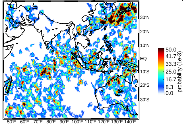
(f) DJF broad strat regions between mod & str thresholds (uw)
