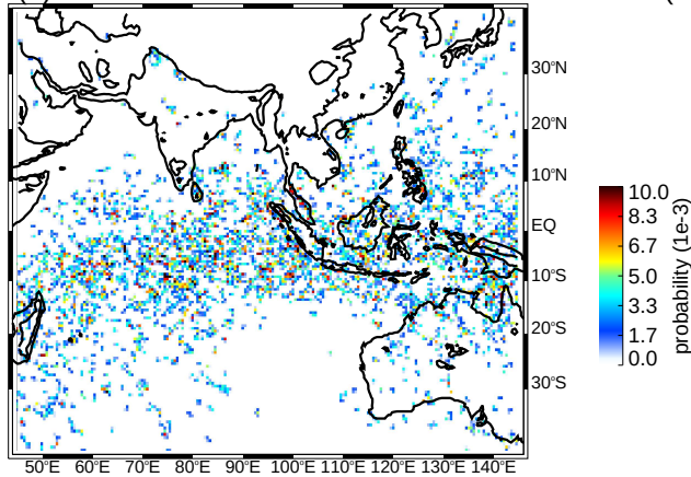
(e) DJF wide convective cores moderate thresholds (uw)
