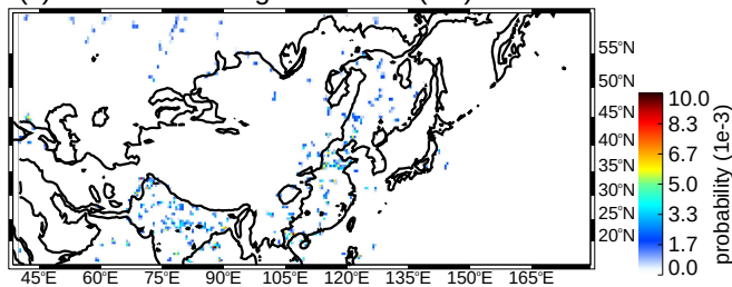
(c) JJA DWC strong thresholds (uw)
