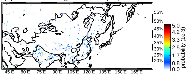
(b) JJA DCC strong thresholds (uw)
