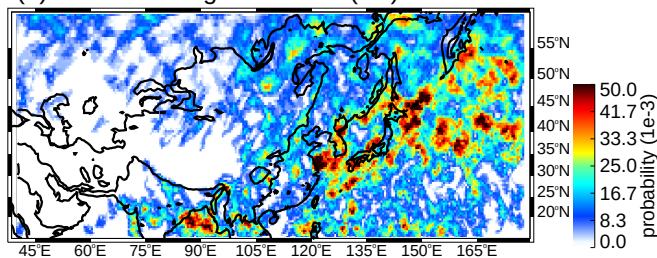
(a) JJA BS strong thresholds (uw)
