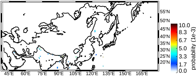
(c) SON DWC strong thresholds (uw)
