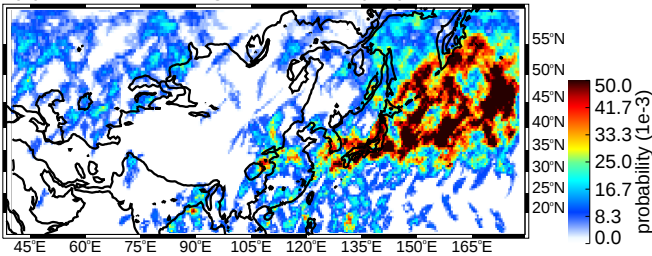
(a) SON BS strong thresholds (uw)
