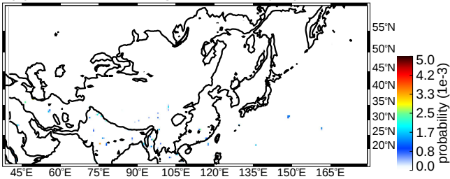
(b) SON DCC strong thresholds (uw)
