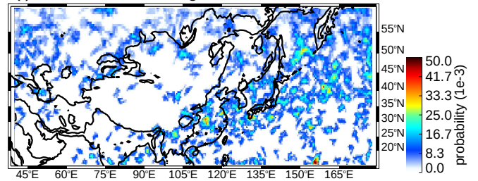
(f) SON broad strat regions between mod & str thresholds (uw)
