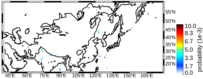
(c) SON deep/wide convective cores strong thresholds (uw)
