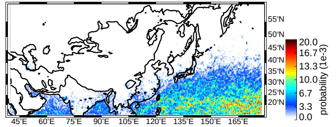
(b) SON shallow isolated cores (uw)
