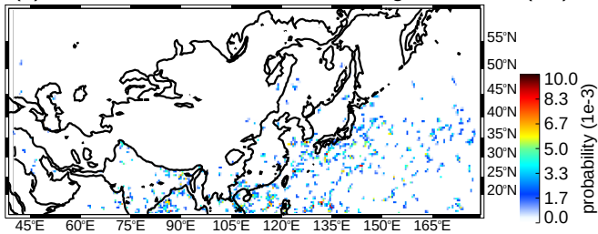
(e) SON wide convective cores strong thresholds (uw)
