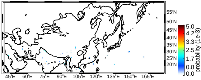
(a) SON deep convective cores strong thresholds (uw)
