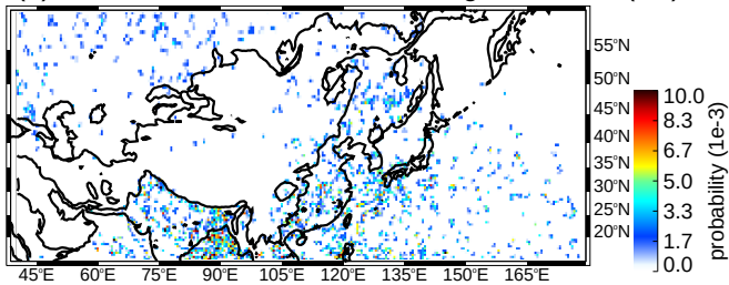
(e) JJA wide convective cores strong thresholds (uw)
