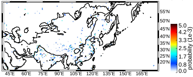
(a) JJA deep convective cores strong thresholds (uw)
