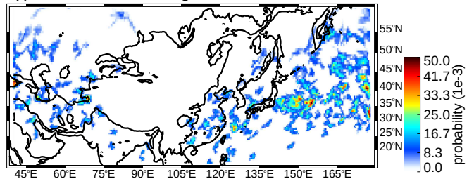
(f) DJF broad strat regions between mod & str thresholds (uw)
