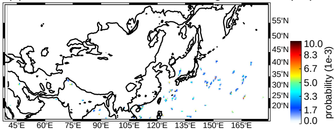
(e) DJF wide convective cores strong thresholds (uw)
