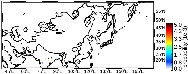
(a) DJF deep convective cores strong thresholds (uw)
