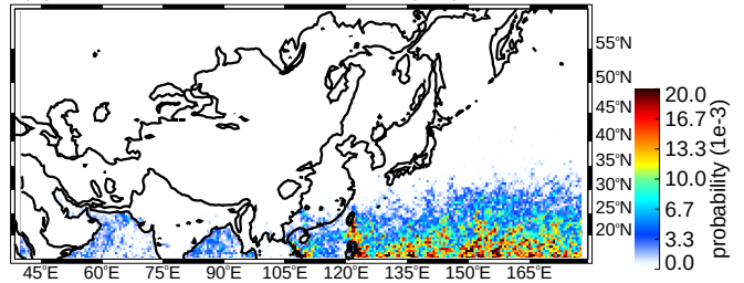
(b) DJF shallow isolated cores (uw)
