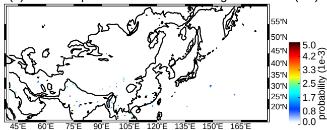
(b) SON deep convective cores strong thresholds (uw)
