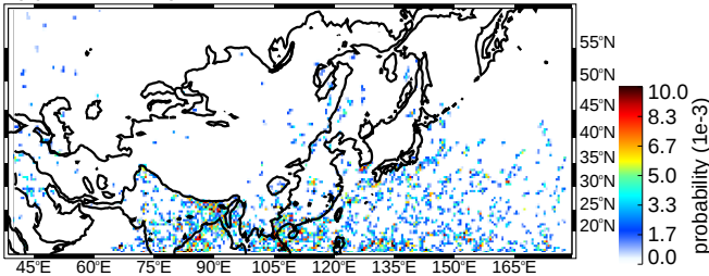
(c) SON deep/wide convective cores moderate thresholds (uw)
