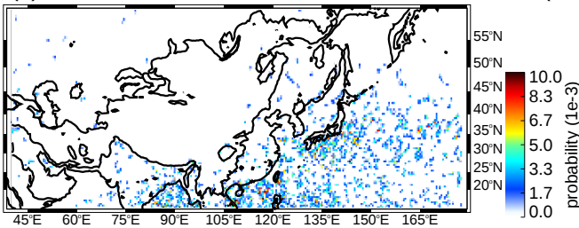
(e) SON wide convective cores moderate thresholds (uw)
