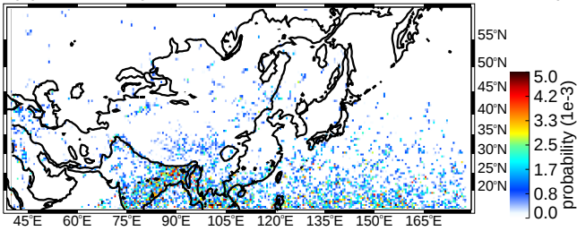
(a) SON deep convective cores moderate thresholds (uw)
