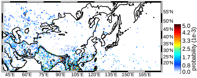
(a) MAM deep convective cores moderate thresholds (uw)
