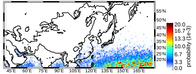
(b) MAM shallow isolated cores (uw)
