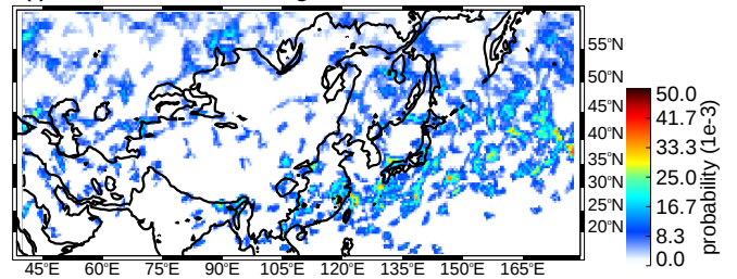
(f) MAM broad strat regions between mod & str thresholds (uw)
