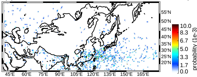
(e) MAM wide convective cores moderate thresholds (uw)
