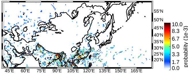
(c) MAM deep/wide convective cores moderate thresholds (uw)
