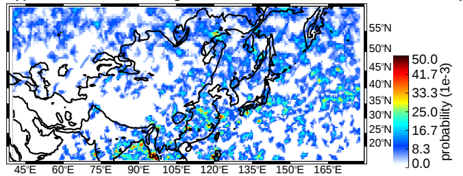
(f) JJA broad strat regions between mod & str thresholds (uw)
