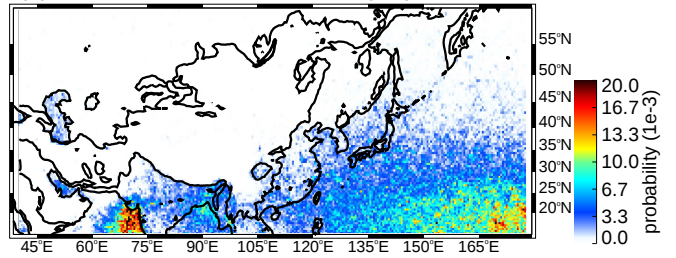
(b) JJA shallow isolated cores (uw)
