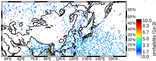
(e) JJA wide convective cores moderate thresholds (uw)
