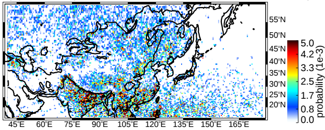
(a) JJA deep convective cores moderate thresholds (uw)
