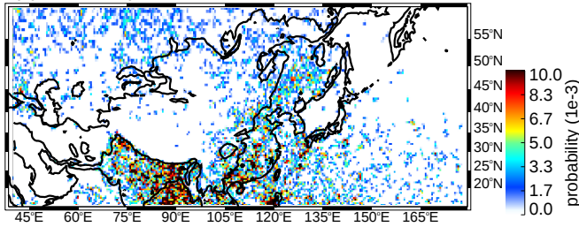
(c) JJA deep/wide convective cores moderate thresholds (uw)
