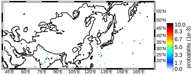
(c) DJF deep/wide convective cores moderate thresholds (uw)
