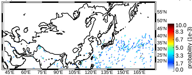
(e) DJF wide convective cores moderate thresholds (uw)
