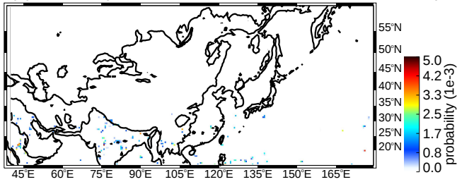
(a) DJF deep convective cores moderate thresholds (uw)
