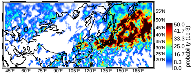
(a) SON broad stratiform regions strong thresholds (uw)
