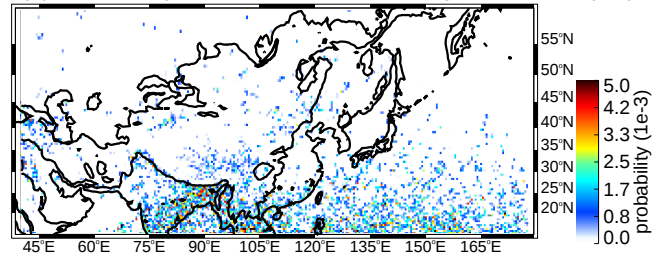
(b) SON deep convective cores strong thresholds (uw)
