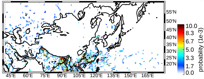
(c) MAM deep/wide convective cores strong thresholds (uw)
