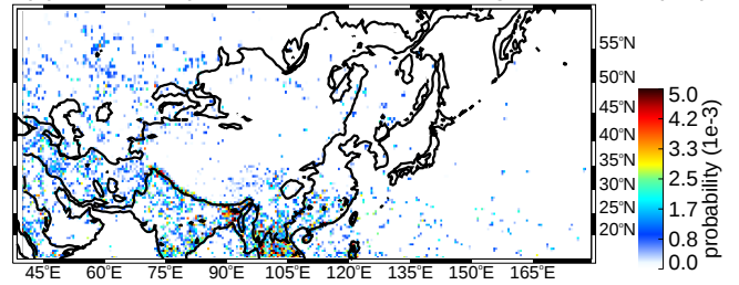
(b) MAM deep convective cores strong thresholds (uw)
