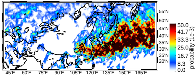
(a) MAM broad stratiform regions strong thresholds (uw)
