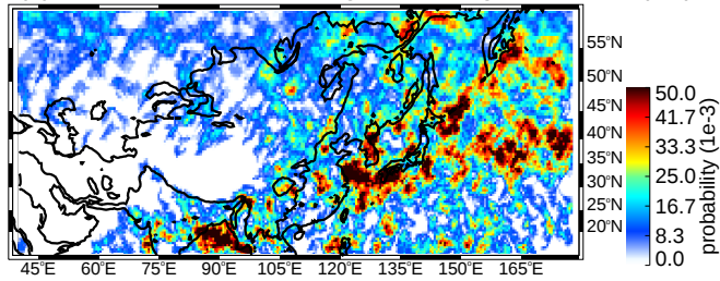
(a) JJA broad stratiform regions strong thresholds (uw)
