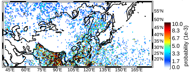
(c) JJA deep/wide convective cores strong thresholds (uw)
