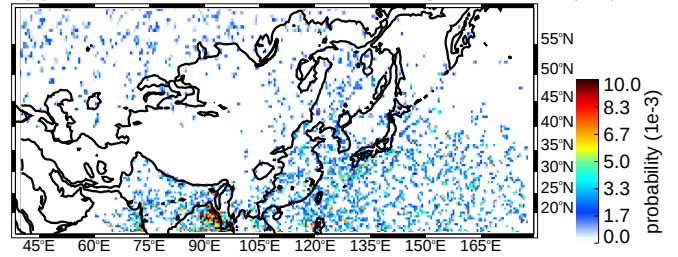
(d) JJA wide convective cores strong thresholds (uw)
