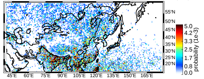
(b) JJA deep convective cores strong thresholds (uw)
