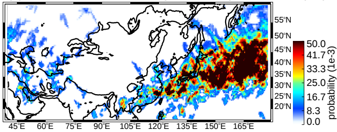
(a) DJF broad stratiform regions strong thresholds (uw)
