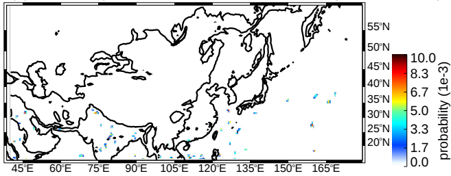
(c) DJF deep/wide convective cores strong thresholds (uw)
