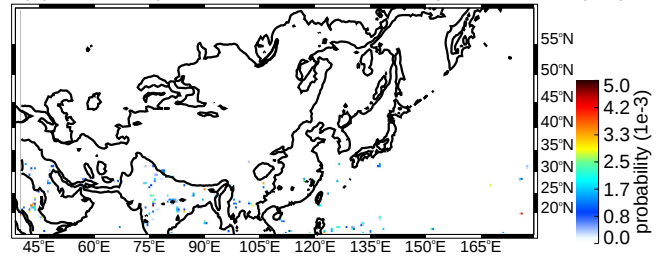
(b) DJF deep convective cores strong thresholds (uw)
