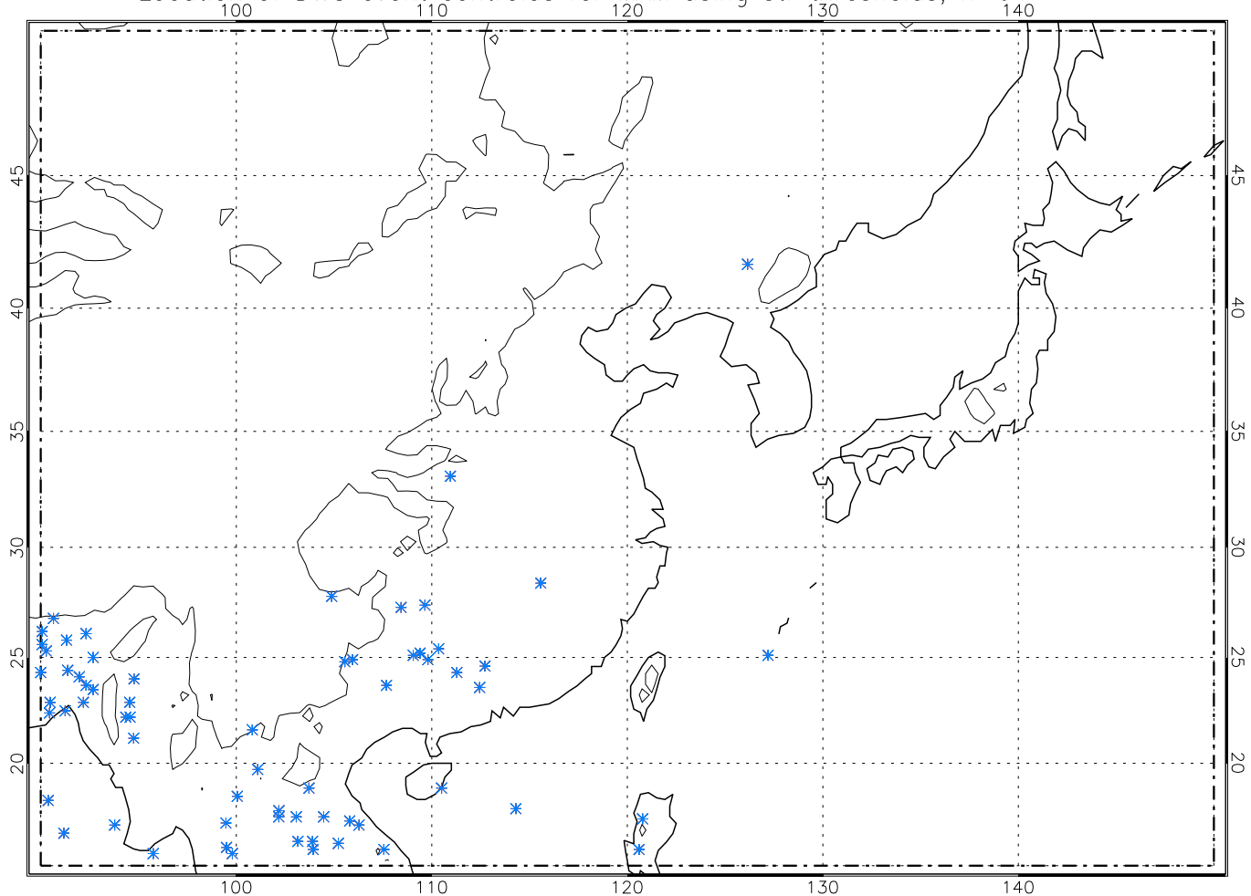
Location of DWC event centroids for MAM using str thresholds, n=64
