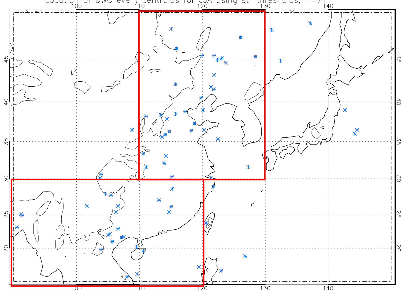
Location of DWC event centroids for JJA using str thresholds, n=71
