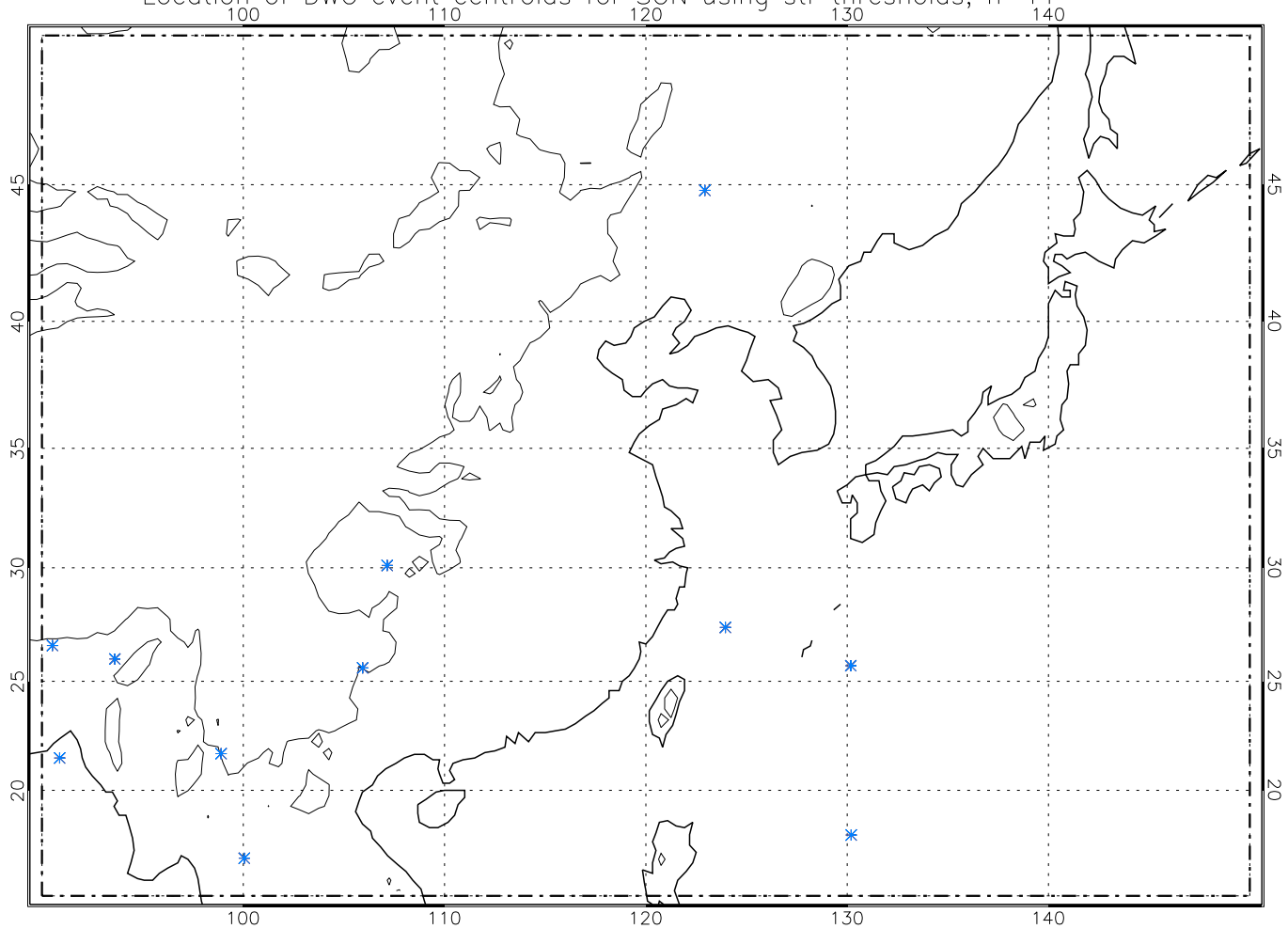
Location of DWC event centroids for SON using str thresholds, n=11
