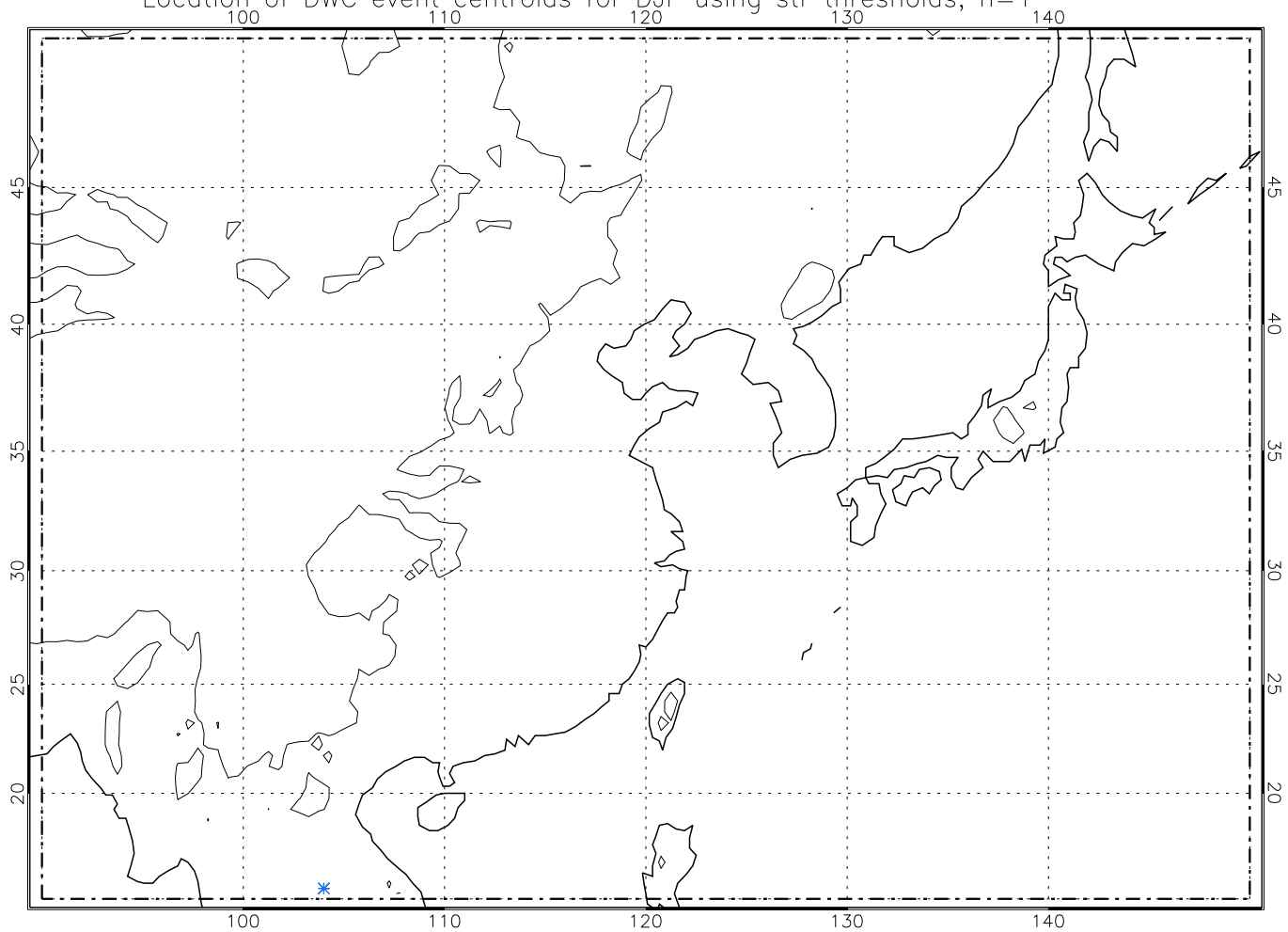
Location of DWC event centroids for DJF using str thresholds, n=1
