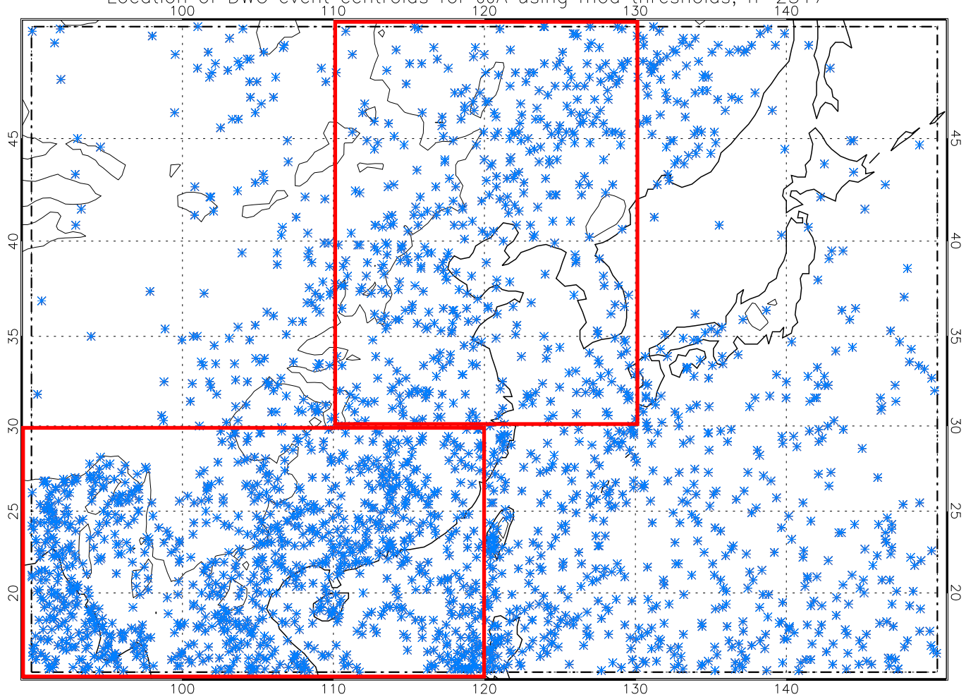
Location of DWC event centroids for JJA using mod thresholds, n=2317
