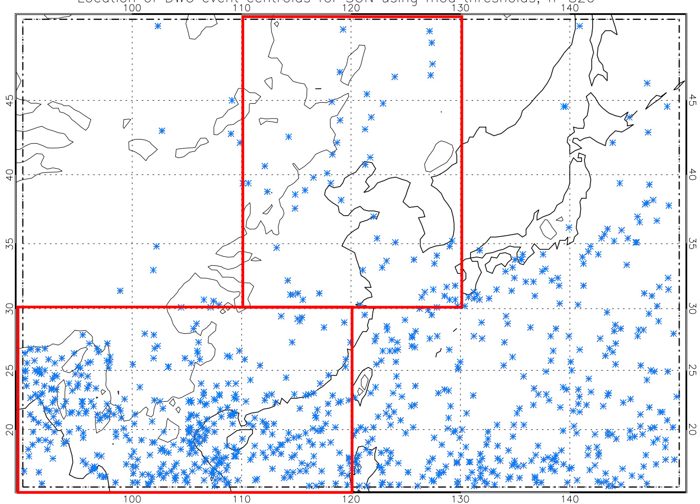
Location of DWC event centroids for SON using mod thresholds, n=820
