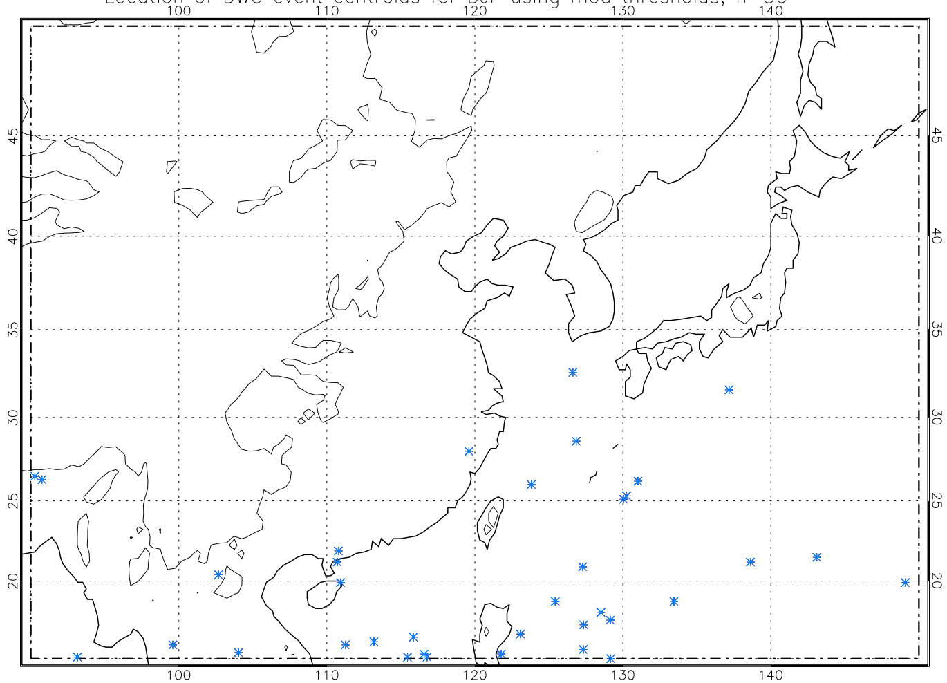
Location of DWC event centroids for DJF using mod thresholds, n=36
