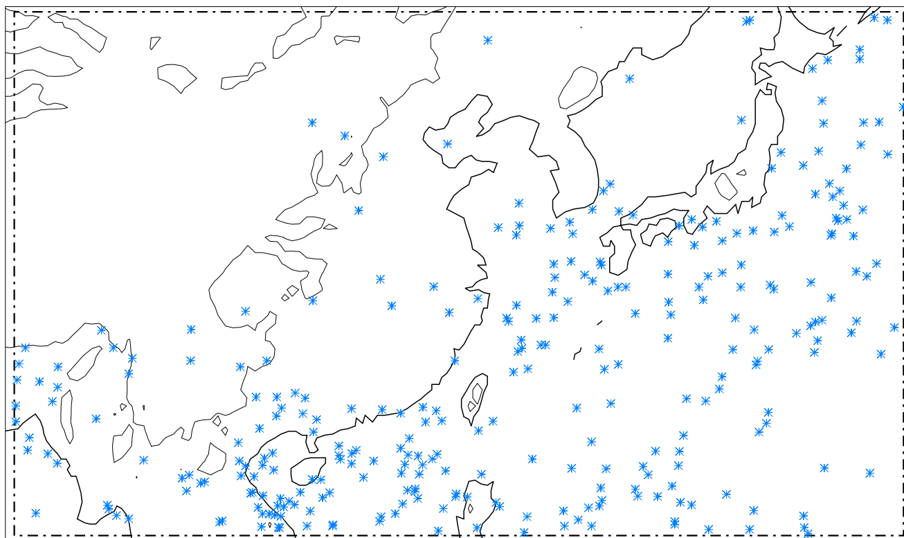
WCC event centroids for CHINA, SON, strong thresholds, nevents=303
