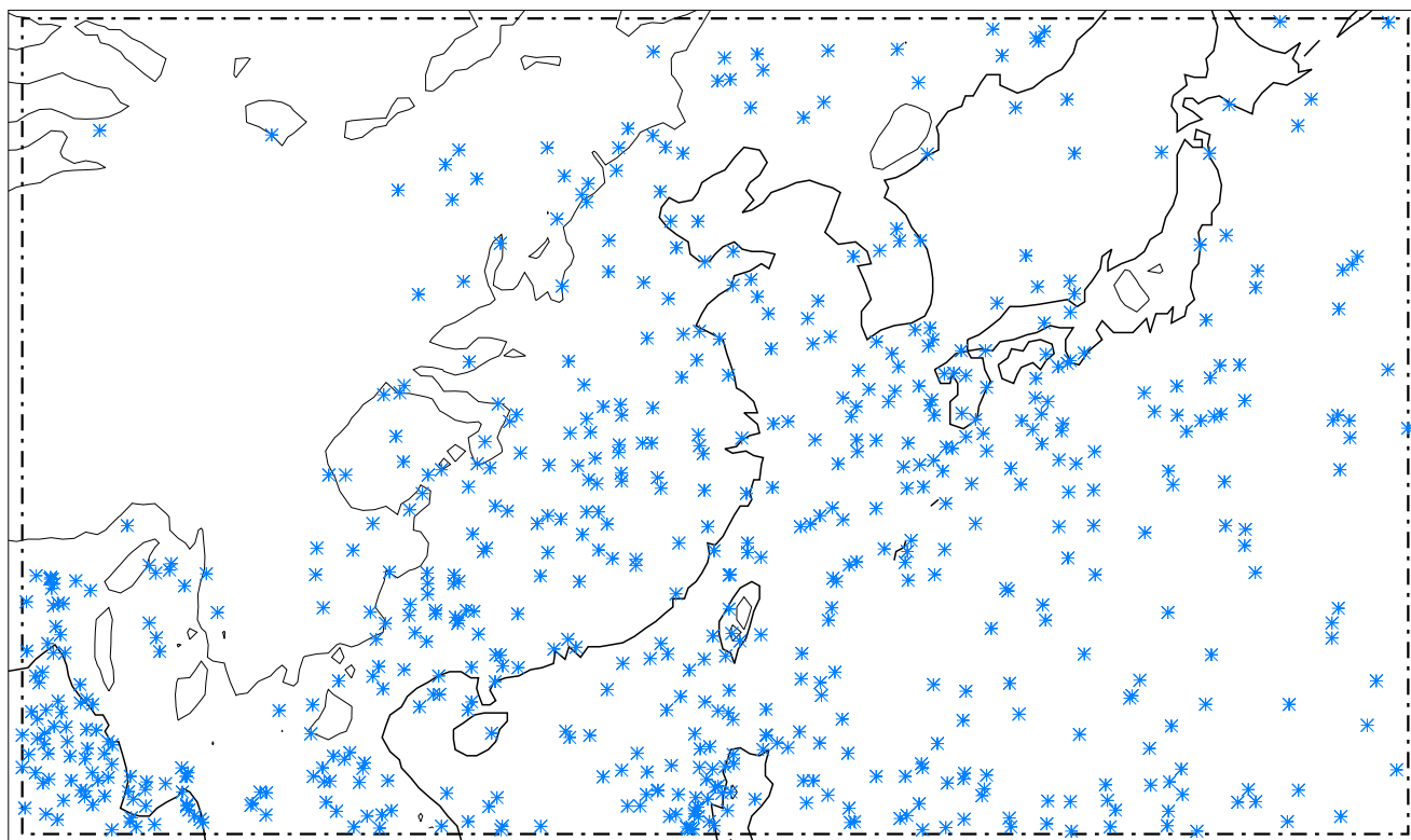
WCC event centroids for CHINA, JJA, strong thresholds, nevents=628
