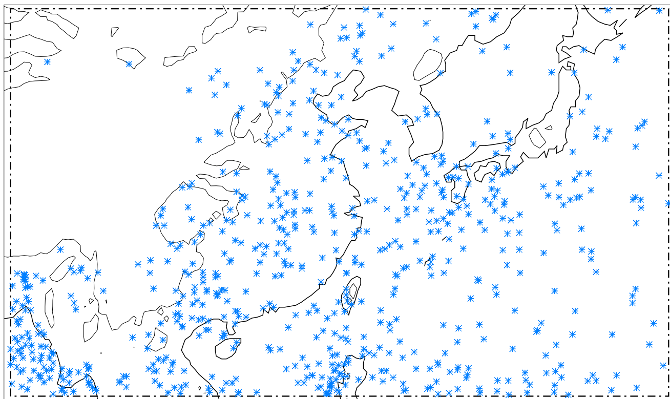
DWC+WCC event centroids for CHINA, JJA, strong thresholds, nevents=690
