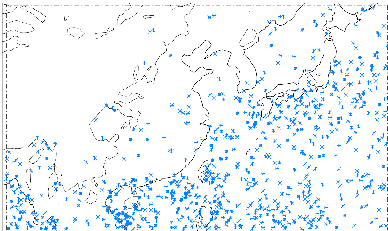
WCC event centroids for CHINA, SON, moderate thresholds, nevents=796
