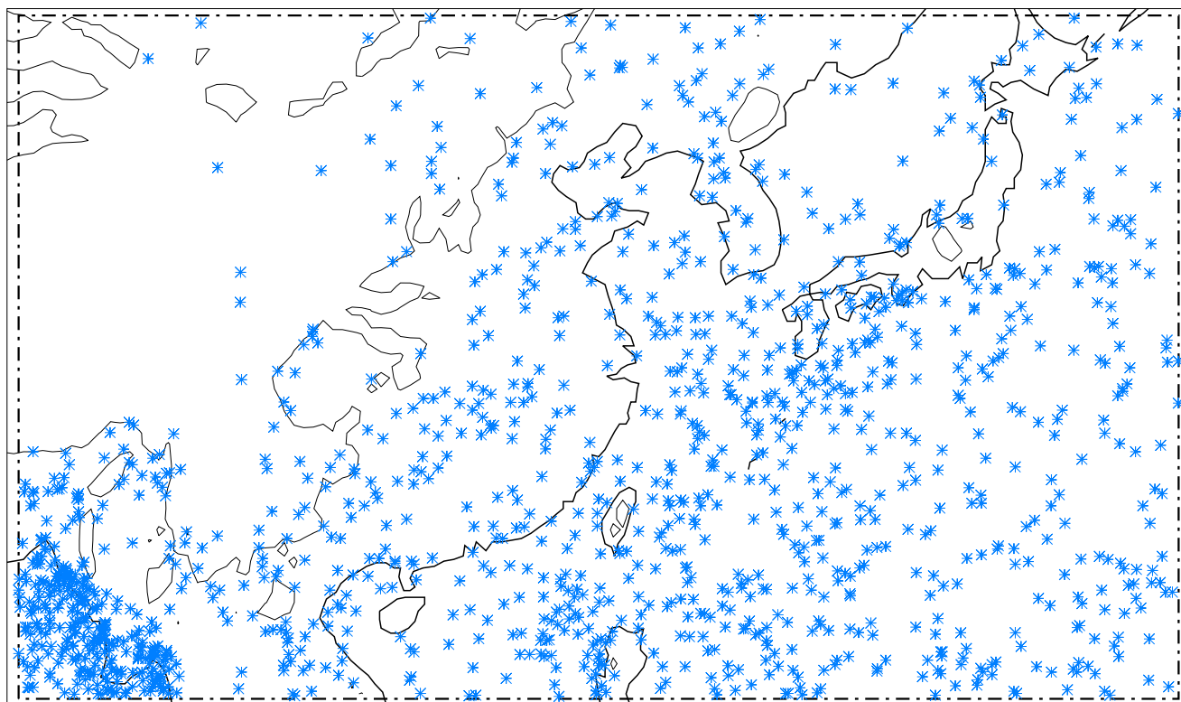
WCC event centroids for CHINA, JJA, moderate thresholds, nevents=1294
