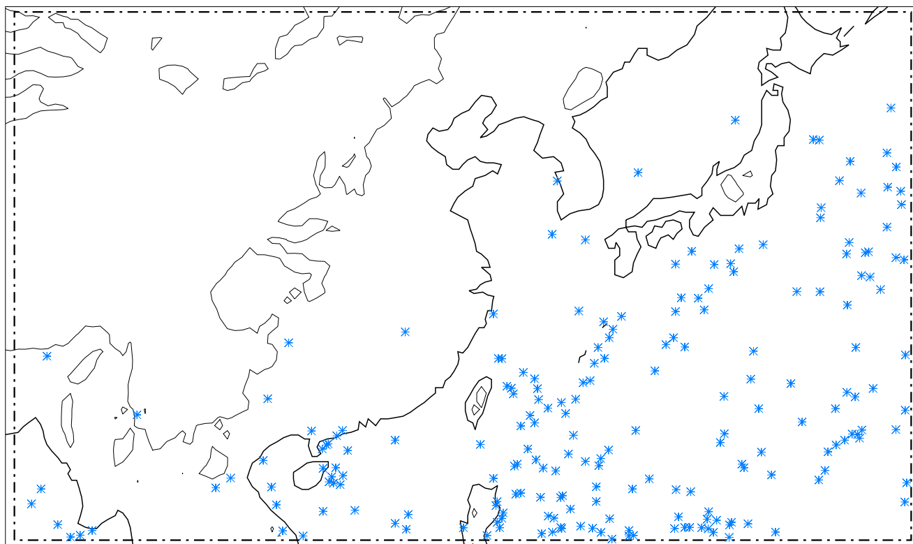
WCC event centroids for CHINA, DJF, moderate thresholds, nevents=207
