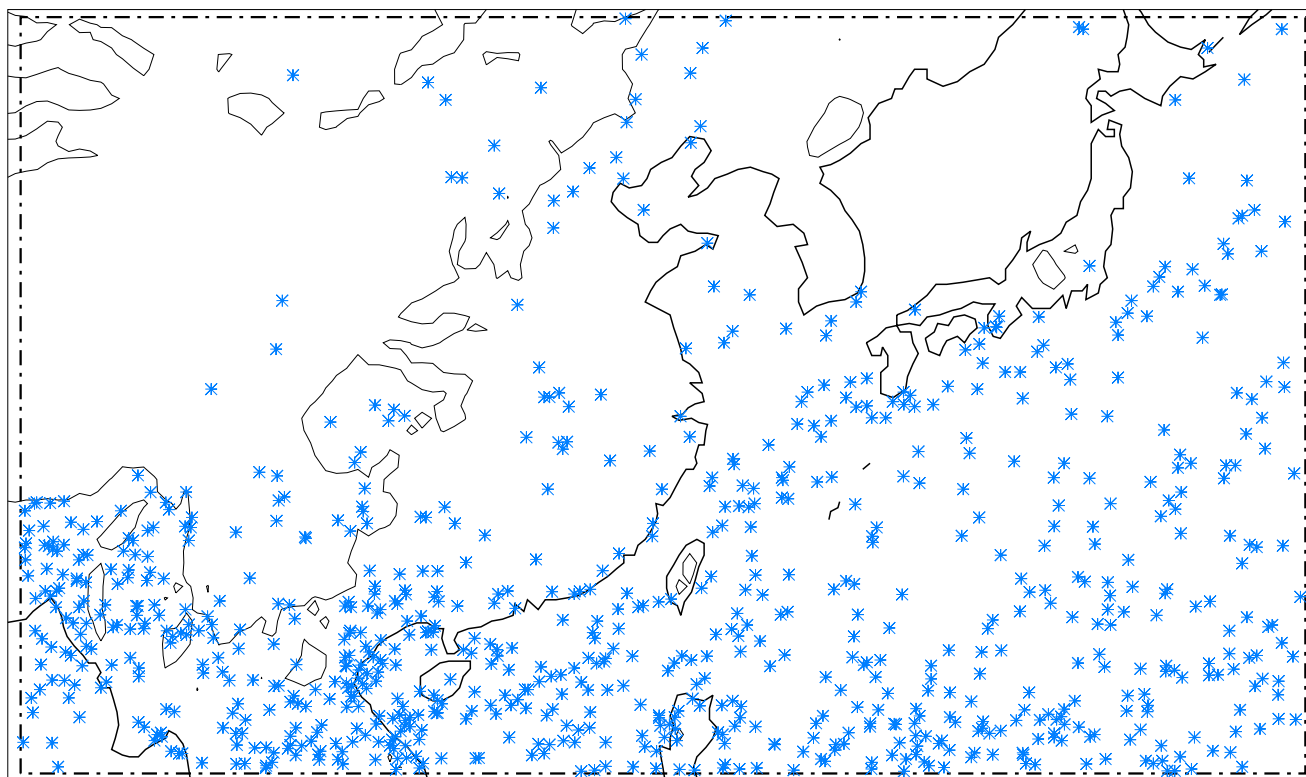
DWC event centroids for CHINA, SON, moderate thresholds, nevents=808
