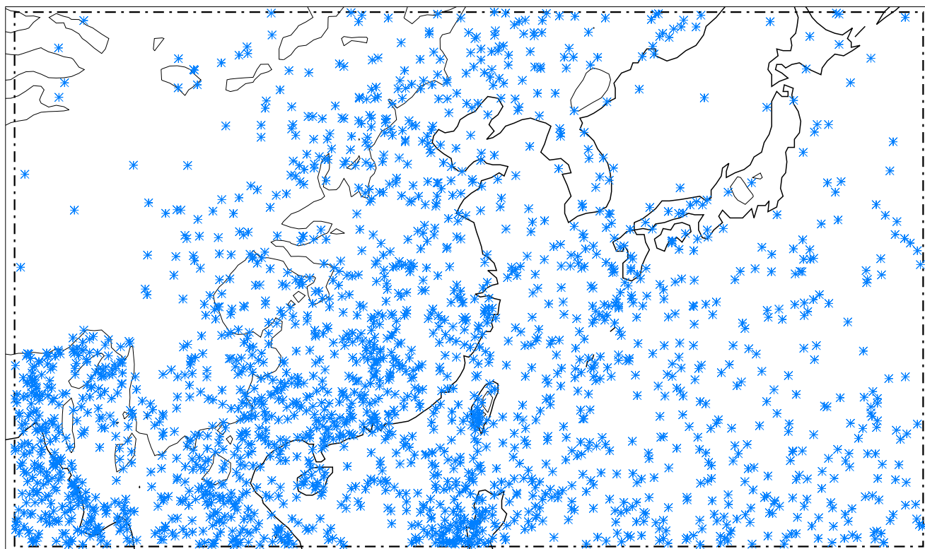
DWC event centroids for CHINA, JJA, moderate thresholds, nevents=2093
