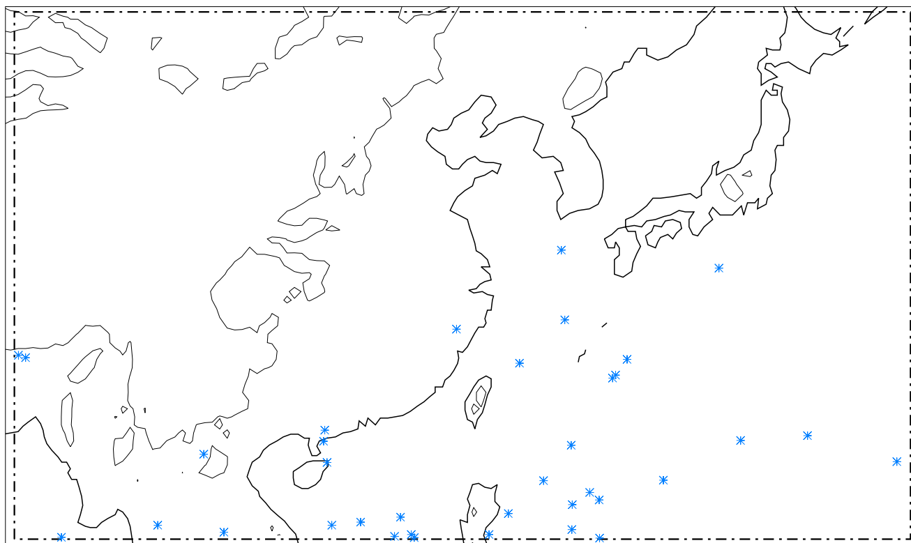
DWC event centroids for CHINA, DJF, moderate thresholds, nevents=36
