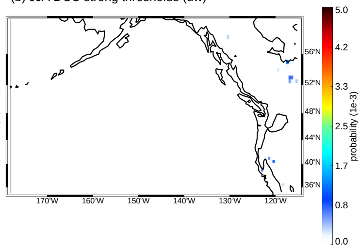
(b) JJA DCC strong thresholds (uw)
