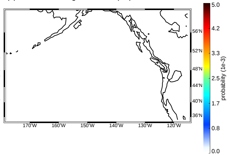
(b) DJF DCC strong thresholds (uw)
