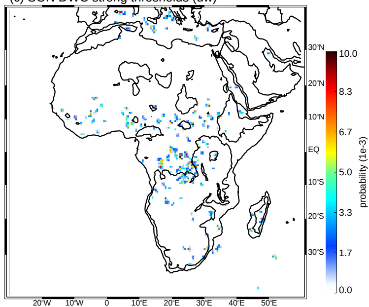
(c) SON DWC strong thresholds (uw)
