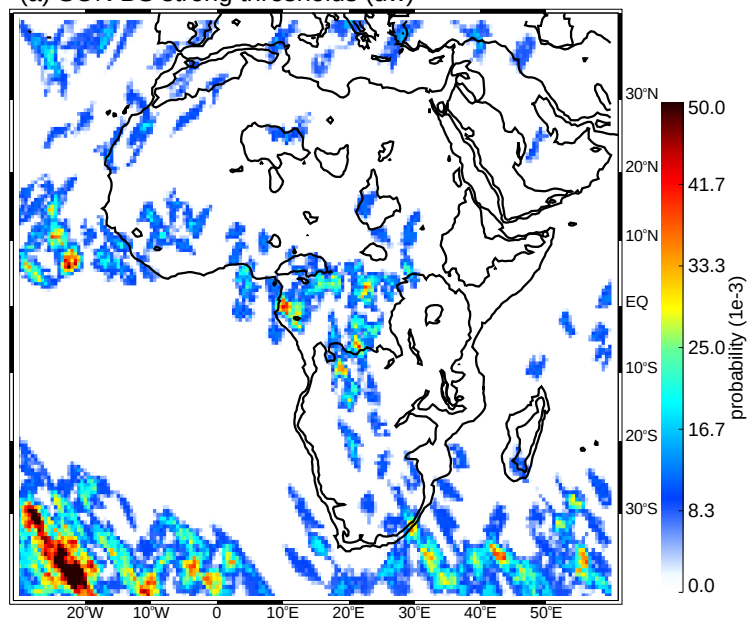
(a) SON BS strong thresholds (uw)
