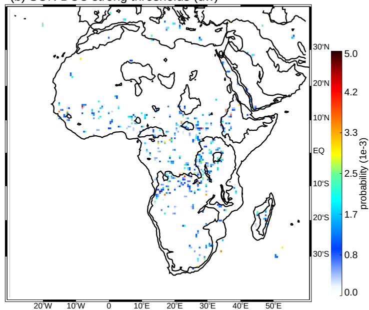
(b) SON DCC strong thresholds (uw)
