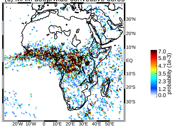
(c) MAM deep/wide convective cores
