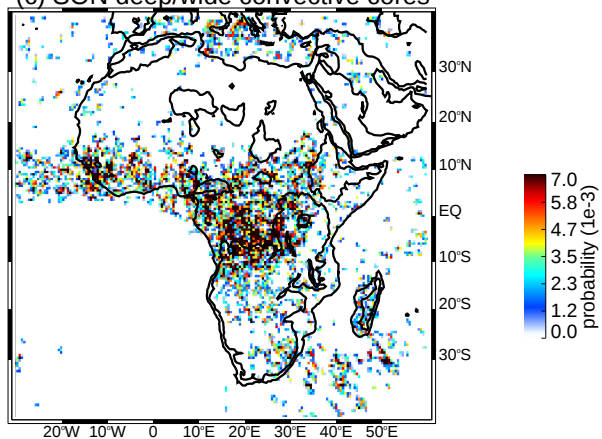
(c) SON deep/wide convective cores
