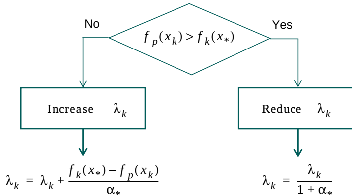
Figure 2-5: Updating \lambda_k
