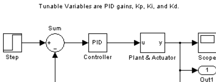
Figure 1-3: Closed-Loop Model
