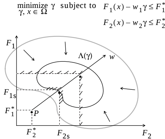
Figure 2-12: Geometrical Representation of Goal Attainment Method
