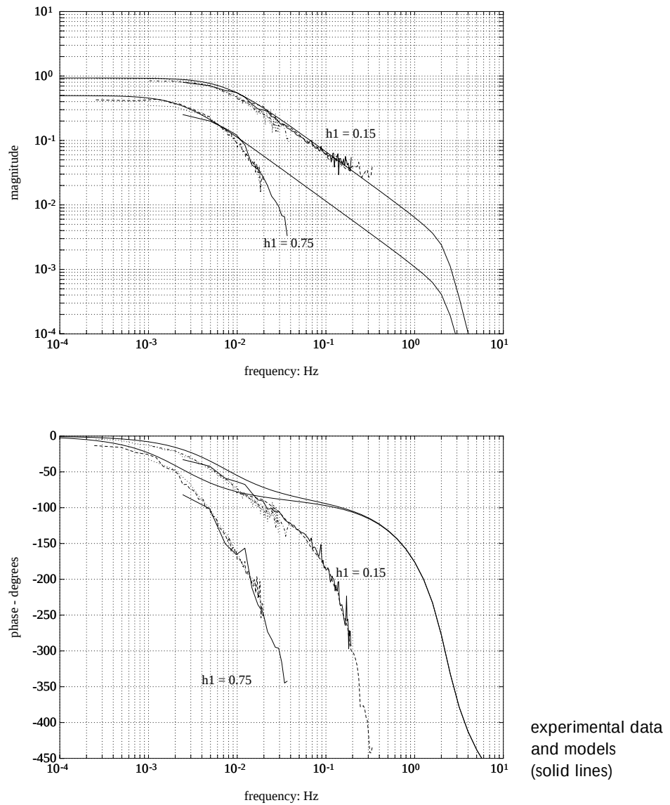
Figure 7-77 Transfer Function Between f_{hc} - f_{cc} and t_1 . Experimental Data and Models. h_1 = 0.15 and h_1 = 0.75 .
