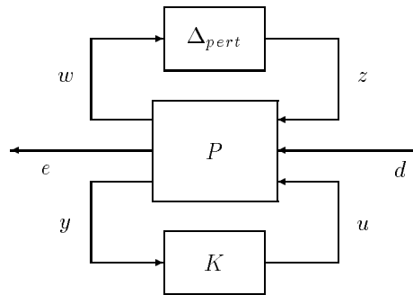
Figure 5-1 LFT Description of Control Problem
