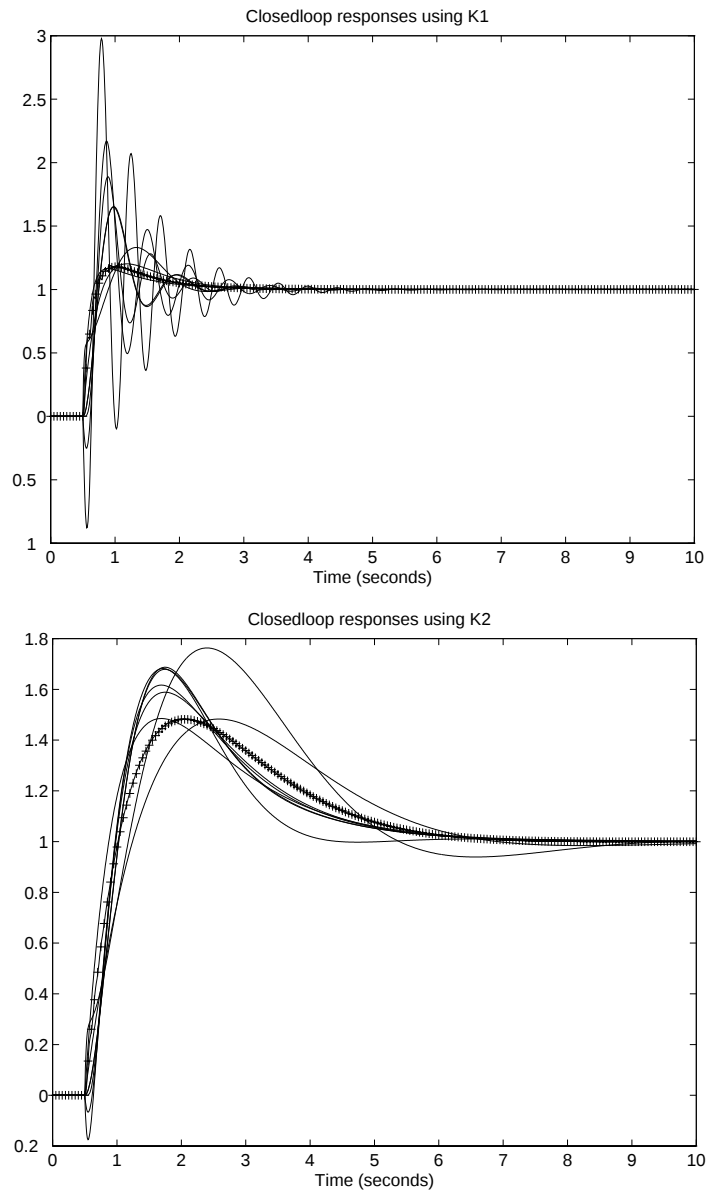
Figure 7-19 Time Response with K1 (top) and K2 (bottom) Implemented
