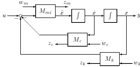
Figure 4-3 Known Part of Uncertain System
