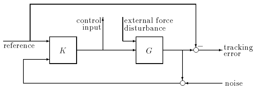
Figure 3-1 Typical Closed-Loop Performance Objectives
