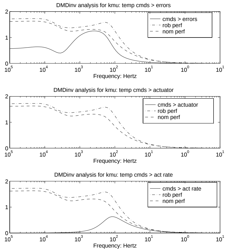
Figure 7-91 DMD^{-1} Analysis for Temperature Reference Command Inputs
