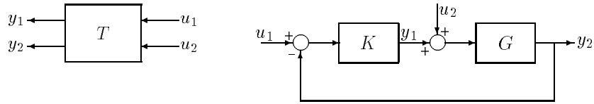
Figure 7-1 formloop Interconnection Structure
