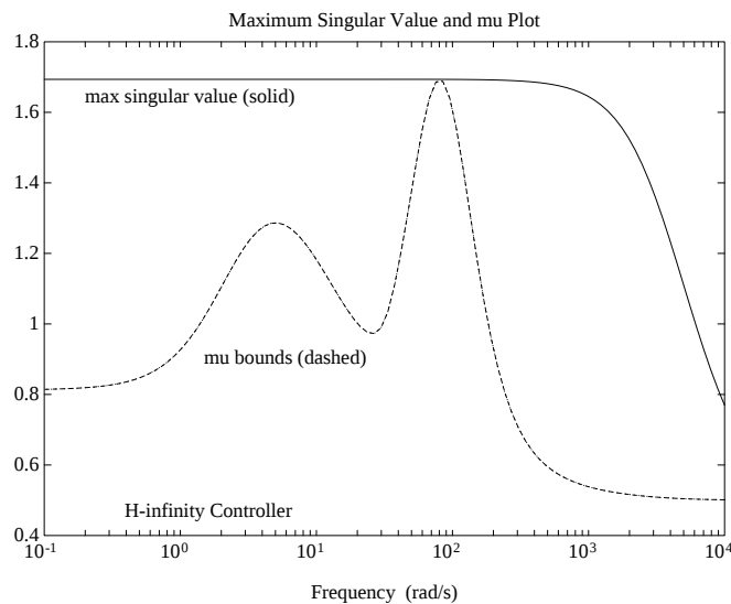
Figure 7-57 Maximum Singular Value of the 4 \times 4 Closed-Loop Transfer Function F_L(P,K_1)(j\omega) and Robust Performance \mu
