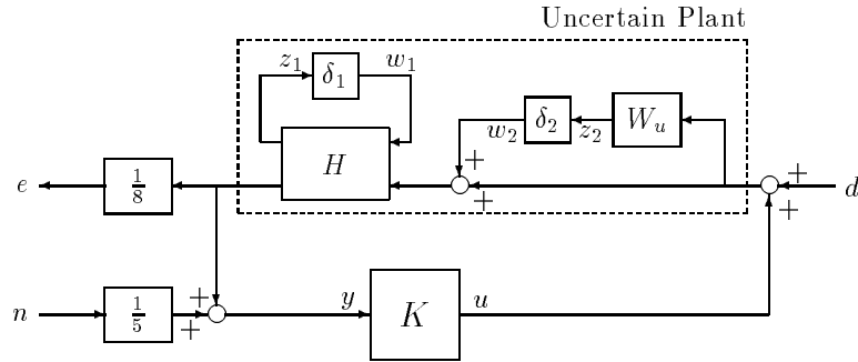
Figure 4-16 Robust Stability/Performance Example
