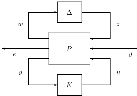
Figure 6-37 Standard Linear Fractional Model
