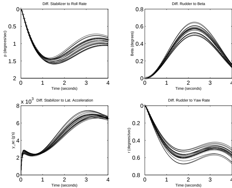
Figure 7-70 Unit Step Responses of the Nominal Model (+) and 15 Perturbed Models from G
