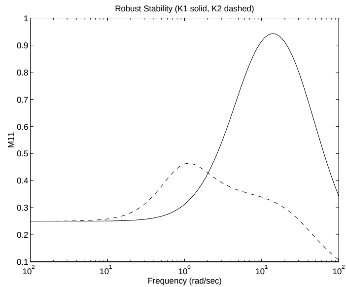
Figure 7-15 Robust Stability Plots
