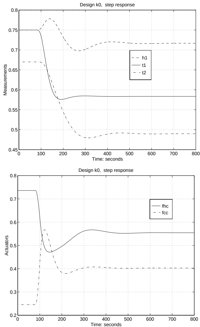
Figure 7-87 Time Response for the Nominal H_\infty Controller
