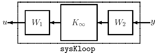
Figure 7-64 Actual Implemented H_\infty Loop Shaping Controller
