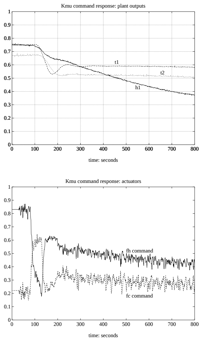
Figure 7-96 Experimental Command Response: Controller K_{mu} with Input Temperature Ramps Going from t_1 = 0.75 , t_2 = 0.67 at 80 Seconds to t_1 = 0.55 , t_2 = 0.47 at 100 Seconds
