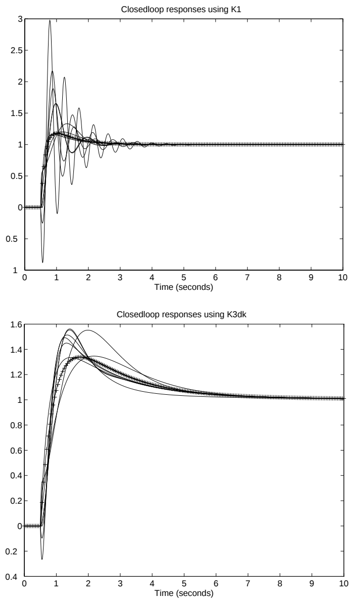
Figure 7-22 Time Response with K1dk (top) and K3dk (bottom) Implemented
