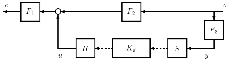
Figure 3-8 Sampled-data System Block Diagram for Simple Example
