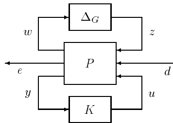
Figure 7-13 General Interconnection for Uncertain System
