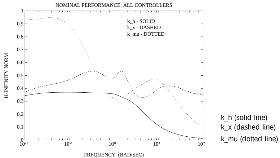
Figure 7-36 Nominal Performance of k_h , k_x , and k_{\mu}
