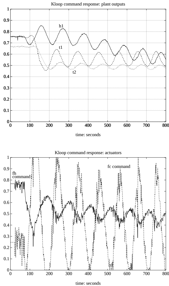
Figure 7-95 Experimental Command Response: Controller K_{loop} with Input Temperature Ramps Going from t_1 = 0.75 , t_2 = 0.67 at 80 Seconds to t_1 = 0.55 , t_2 = 0.47 at 100 Seconds
