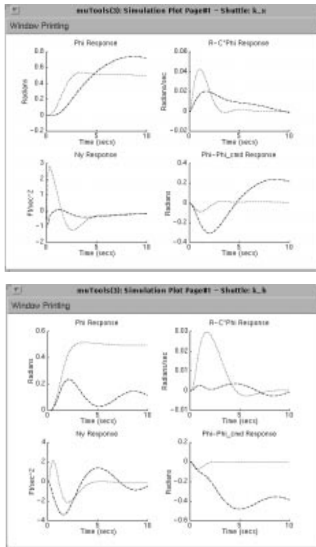
Figure 7-45 Closed-Loop Nominal and Perturbed Time Response, k_x (top) and k_h
