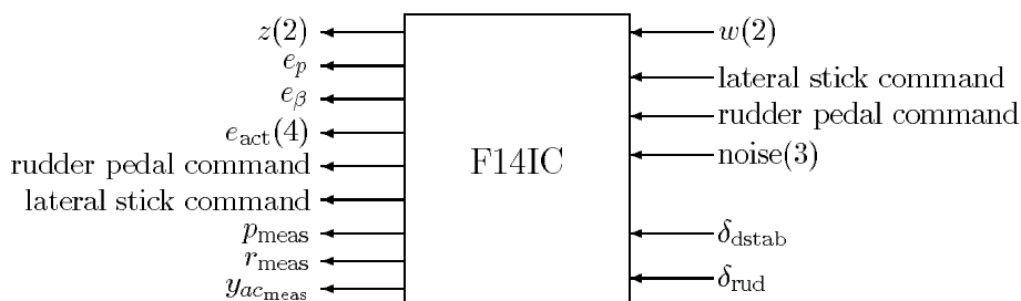
Figure 7-71 F-14 Generalized Plant
