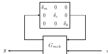
Figure 4-5 Uncertain Mass/Damper/Spring System as LFT
