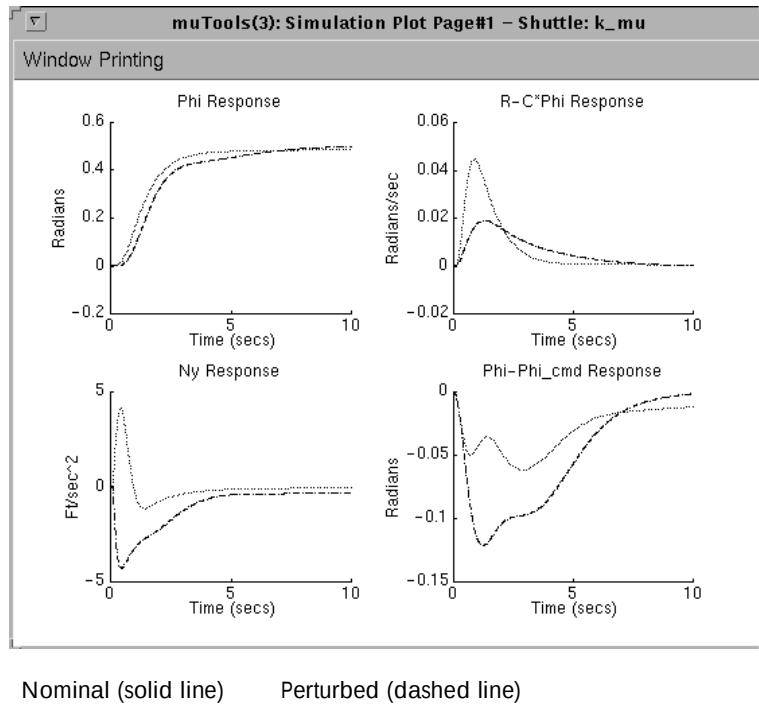
Figure 7-46 Closed-Loop Nominal and Perturbed Time Response, k_{\mu}
