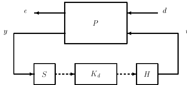
Figure 3-7 Sampled Data System Block Diagram
