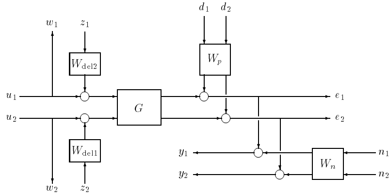
Figure 6-15 Spinning Satellite Interconnection Structure
