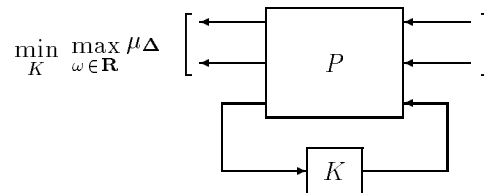
Figure 5-3 \mu Synthesis
