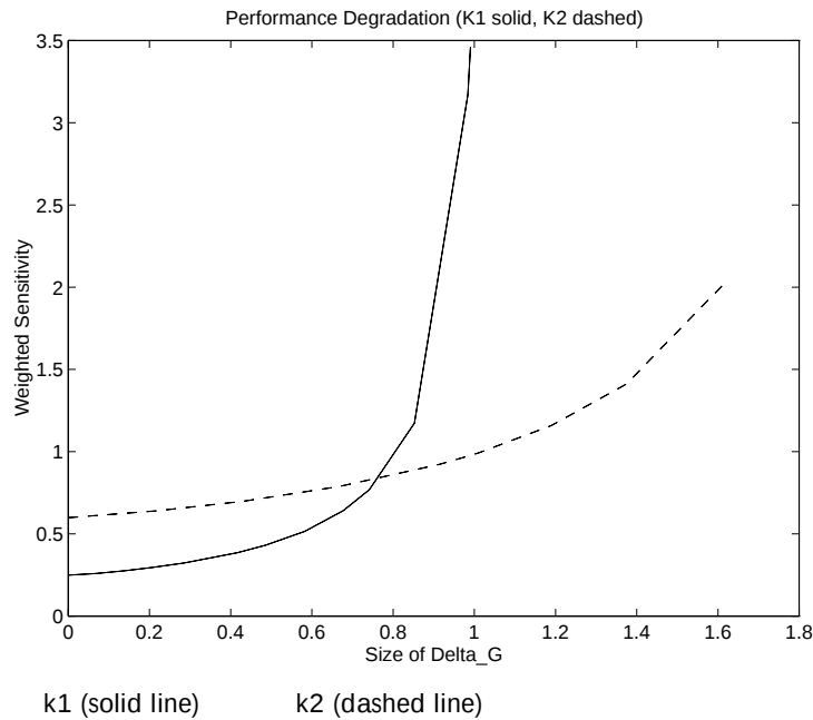
Figure 7-17 Performance Degradation
