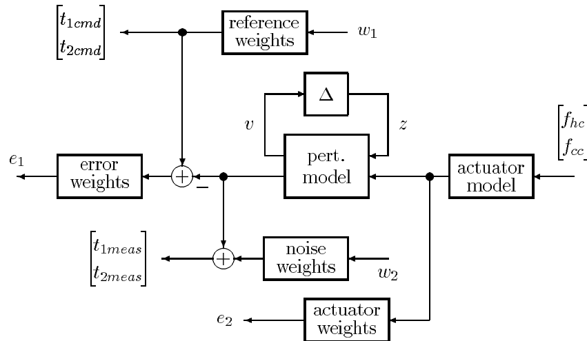
Figure 7-82 Interconnection Structure for the Design Problem
