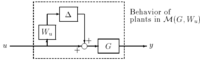
Figure 4-11 Multiplicative Uncertainty
