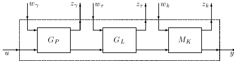
Figure 4-9 Cascade of Pade, Lag, and Gain LFTs
