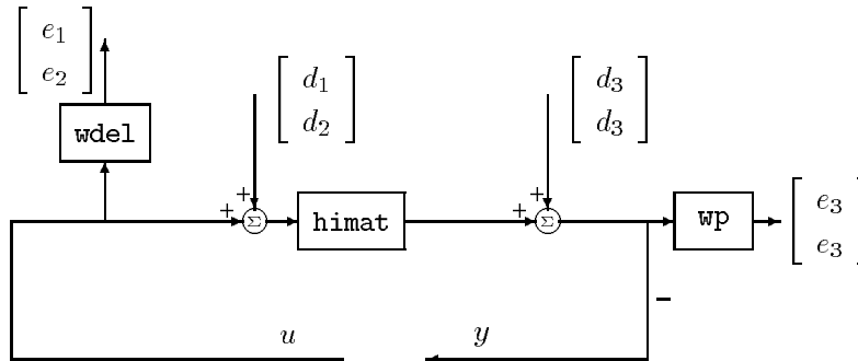
Figure 3-6 H_\infty Design Example Interconnection Structure
